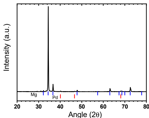
Figure 19. X-ray diffraction pattern of Mg–Pd 2.5 at% after 20 rolling passes. Cu K\alpha radiation.
