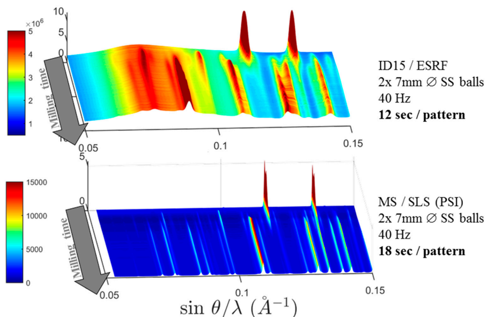
Figure 26. Comparison of XRD patterns collected during the mechanochemical reaction between \text{LiBH}_4 and \text{CsBH}_4 , taken at high energy ESRF beamline (former ID15, 90 keV) and at medium energy MS beamline at SLS (16 keV) [256].
