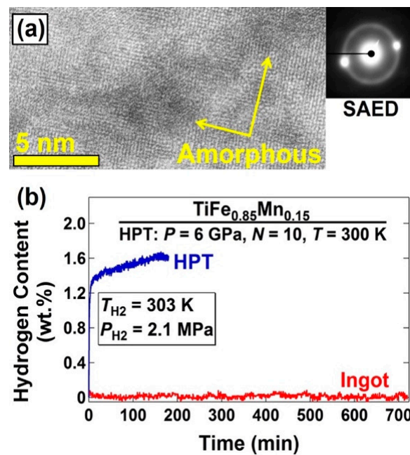
Figure 13. (a) TEM image and corresponding SEAD pattern with nano-sized amorphous regions indicated by arrows; and (b) hydrogenation kinetic curves for \text{TiFe}_{0.85}\text{Mn}_{0.15} after ingot casting and HPT processing [165] (reproduced with permission).
